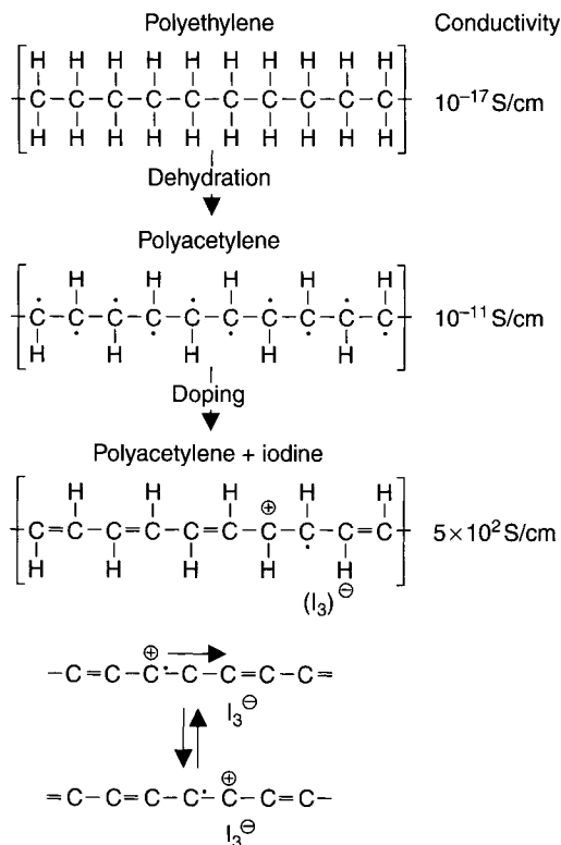
Figure 2.35 Synthesis of polyacetylene and changes in its conductivity on doping with iodine [15].
