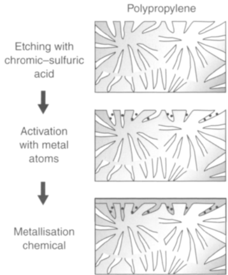
Figure 7.9 Etching, activation and electroless metallising of a polypropylene substrate [8].
